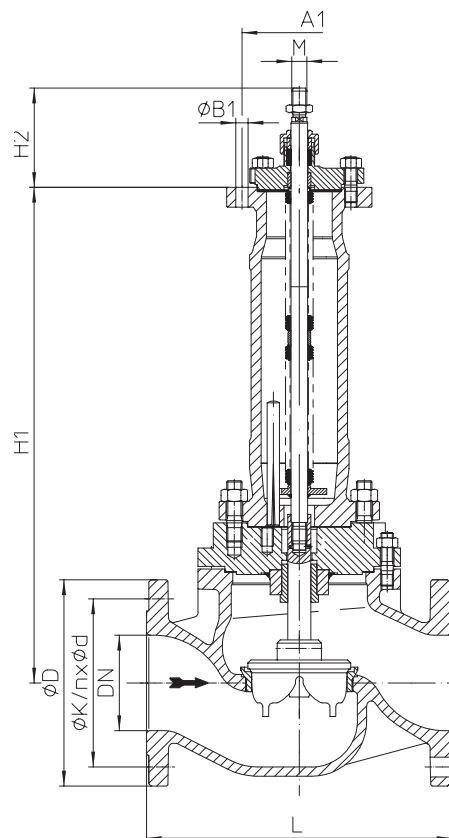
Fig. 471...90 DN200 M20 (e.g.: DP34-34Tri)
