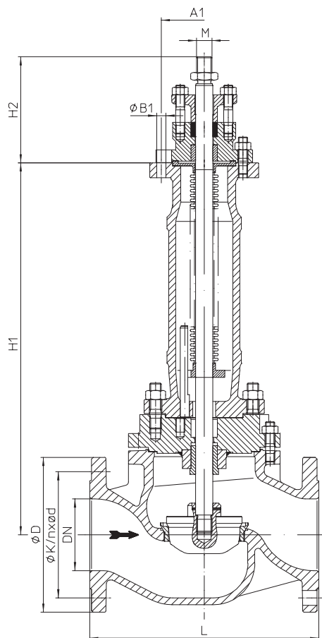
Fig. 471...90 DN150 (e.g.: DP34T-35; AUMA 14.2)
