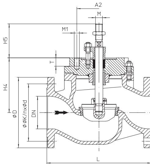
Fig. 470...90 DN150-200 (e.g.: DP35; AUMA 14.2-14.6)
