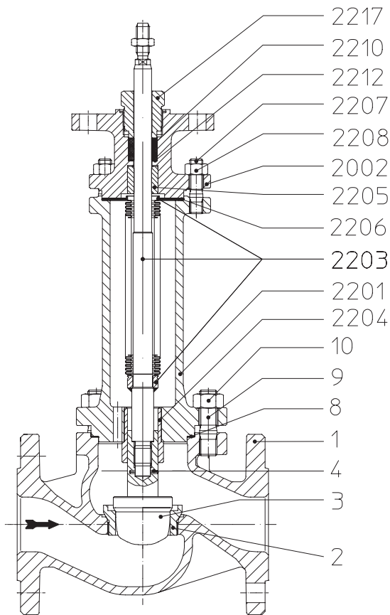
III. PTFE-packing / Pure graphite-packing
